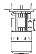
Foot and flange mounted motor. Shaft up.
