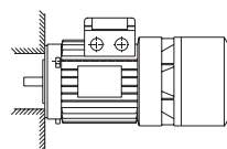
Face mounted. Flange with threaded holes and spigot
